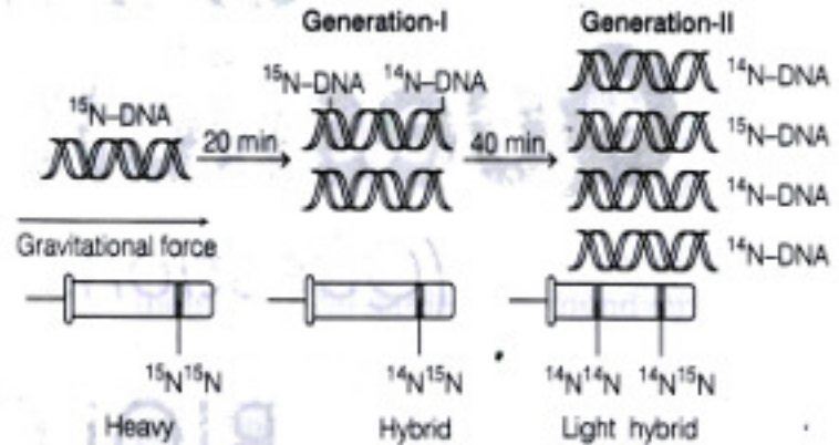
Meselson and Stahl's experiment (5)
